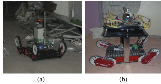
Fig. 4 The three robots used in the experiments include the Kenaf (Fig. 4(a)) and Quince (Fig. 4(b)) tracked ground robots. Here we see the Quince transporting the Pelican between discrete sites of interest via the landing pad.
