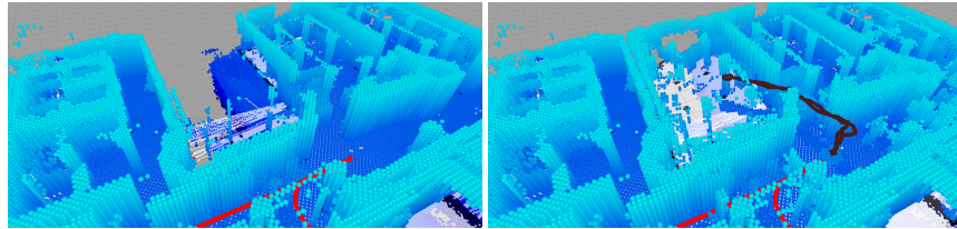
Fig. 11 Merging the Kenaf and Pelican maps. The map generated by the Kenaf is shown on the left while the extended map via the Pelican observations along with the Quince and Pelican trajectories (red and black, respectively) are shown on the right.
