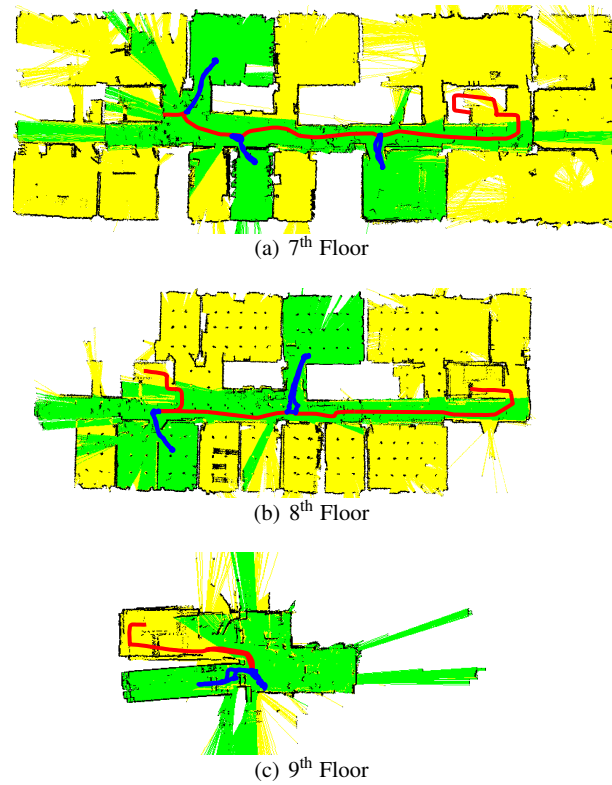
Fig. 9 The 2D occupancy grid maps generated during the experiment of the 7 th , 8 th , and 9 th stories of the Tohoku University Electrical Engineering Building. The contributions to the map made by the Kenaf are shown in yellow with an overlay of the contributions made by the Pelican in green. The path of the Quince is shown in red while the trajectory followed by the Pelican is depicted in blue. The path of the Kenaf is not shown.
