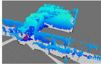
Fig. 8 A representative 3D map generated by the aerial vehicle during flight. A 2D occupancy grid map is also generated at all times. The vehicle and its path are shown as a red mesh and line, respectively.
