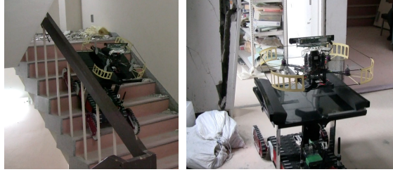
Fig. 3 The Quince ground platform carries the Pelican aerial robot via a landing pad. The aerial robot opens and closes the landing pad via a wireless interface during autonomous take-off and landing. A video of the experiment is available at http://mrsl.grasp.upenn.edu/nmichael/fsr2012.mov .
