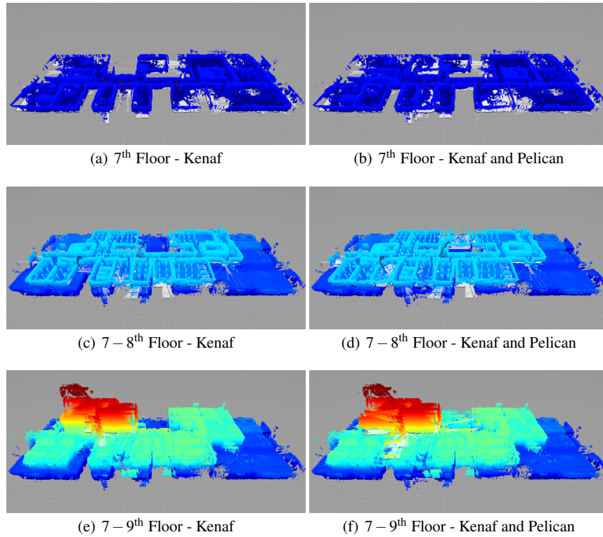
Fig. 10 The 3D voxel grid maps generated during the experiment. The map resulting from the Kenaf sensor data is shown on the left while the merged maps resulting from both the Kenaf and Pelican sensor data are shown on the right.
