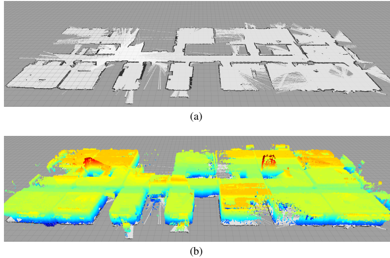
Fig. 6 The 2D occupancy grid map (Fig. 6(a)) and 3D point-cloud map (Fig. 6(b)) of the 7 th floor generated via the Kenaf sensor data.
