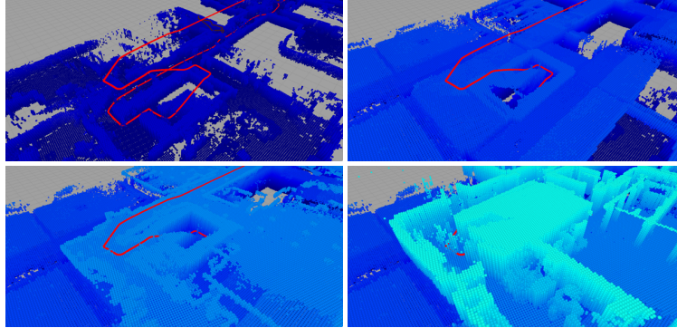
Fig. 12 The 3D map generated for the stairwell traversed by the vehicles between the 7 th and 8 th floors showing various z -height levels of detail along with the trajectory followed by the Quince robot.
