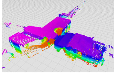
Fig. 7 The 3D rotating laser scanner on the Kenaf generates feature-rich 3D point clouds. Here we show the full output from a single revolution of the scanner.
